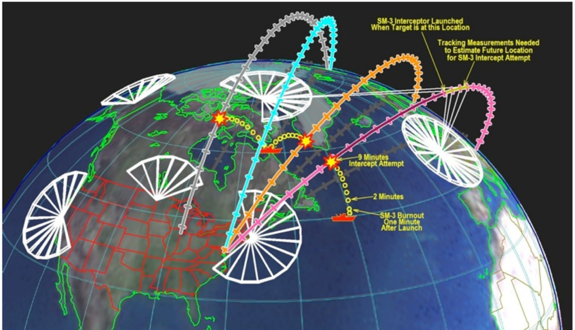
Figure 3: Northwest Atlantic-based SM3 Block II interceptors (with a conservative assumed burnout speed of 4 km/sec) engaging Russian ICBM warheads: each tick on the trajectories marks one minute. 16p280 Defenses, p. 114 FKL, Dep. of Physics © 2016
