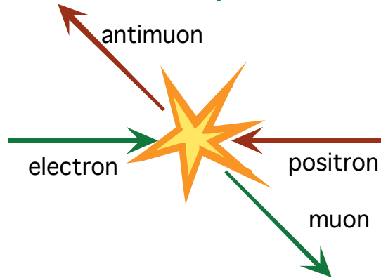
Annihilation process
