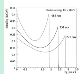
Differential cross sections for the CBS process between 8-GeV electrons and laser photons
