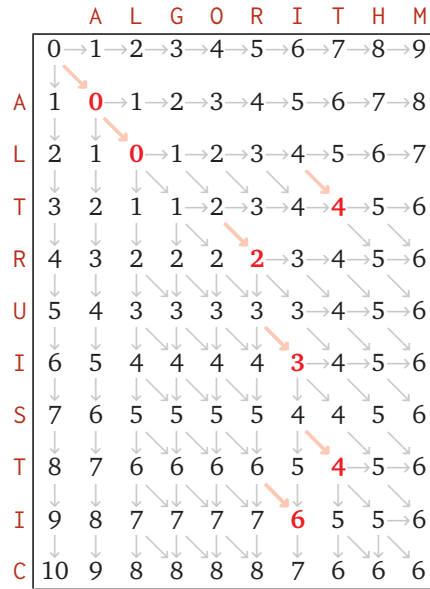
Figure 3.5. The memoization array for Edit(ALGORITHM, ALTRUISTIC)
