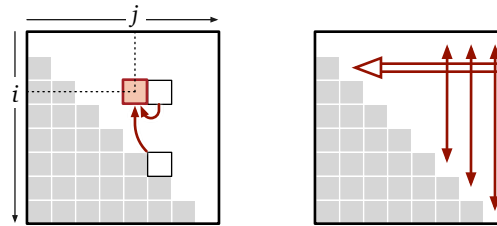
Figure 3.3. Dependencies between subproblems for longest increasing subsequence, and a valid evaluation order
