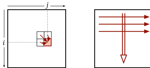
Figure 3.4. Dependencies in the memoization table for edit distance, and a valid evaluation order
