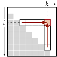
Figure 3.7. Subproblem dependencies in the optimal binary search tree problem.
