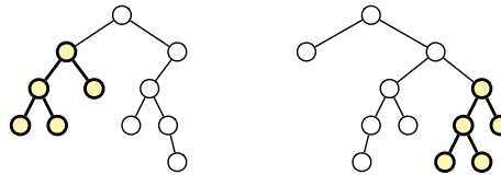
Figure 3.16. Two binary trees, with their largest common (rooted) subtree emphasized.
