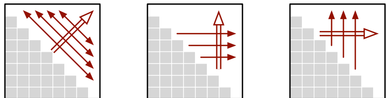
Figure 3.8. Three different evaluation orders for the optimal binary search tree problem.
