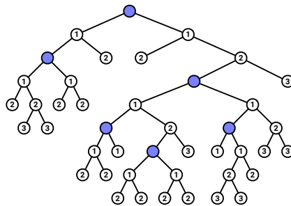
Figure 3.15. A subset of five vertices in a binary tree, with clustering cost 3.
