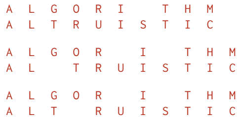
Figure 3.6. Three optimal transformations from ALGORITHM into ALTRUISTIC .
