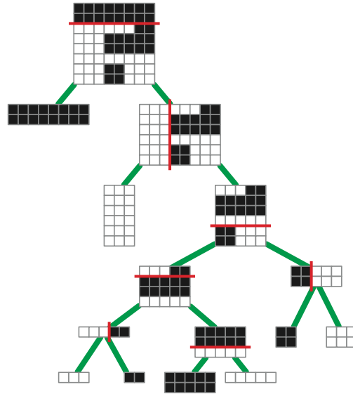
Figure 3.10. A guillotine subdivision with size 8 and depth 5.
