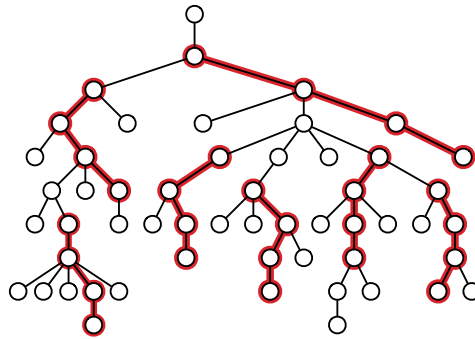
Figure 3.14. Seven disjoint paths of length k = 3 . This is not the largest such set of paths in this tree.
