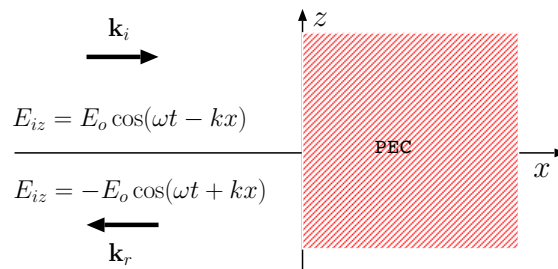
(a) Stationary reflector (in lab frame)
