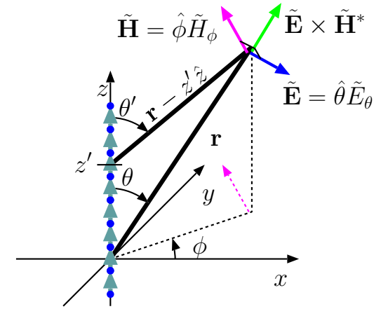
Field due to dipole at the origin
