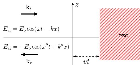
(b) Moving reflector
