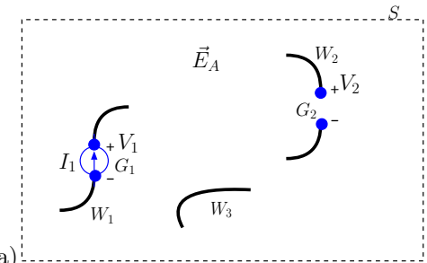
Antenna 1 with input current I_1 causes an open circuit voltage response V_2 at antenna 2 terminals across some distance r (due to field \mathbf{E}_A ).
