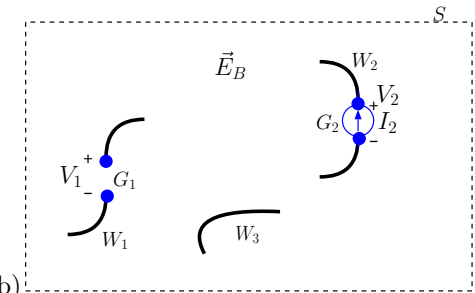
Antenna 2 with input current I_2 causes an open circuit voltage response V_1 at antenna 1 terminals across some distance r (due to field \mathbf{E}_B ).
