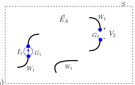
(a) Antenna 1 with input current I_1 causes an open circuit voltage response V_2 at antenna 2 terminals across some distance r (due to field \mathbf{E}_A ).
