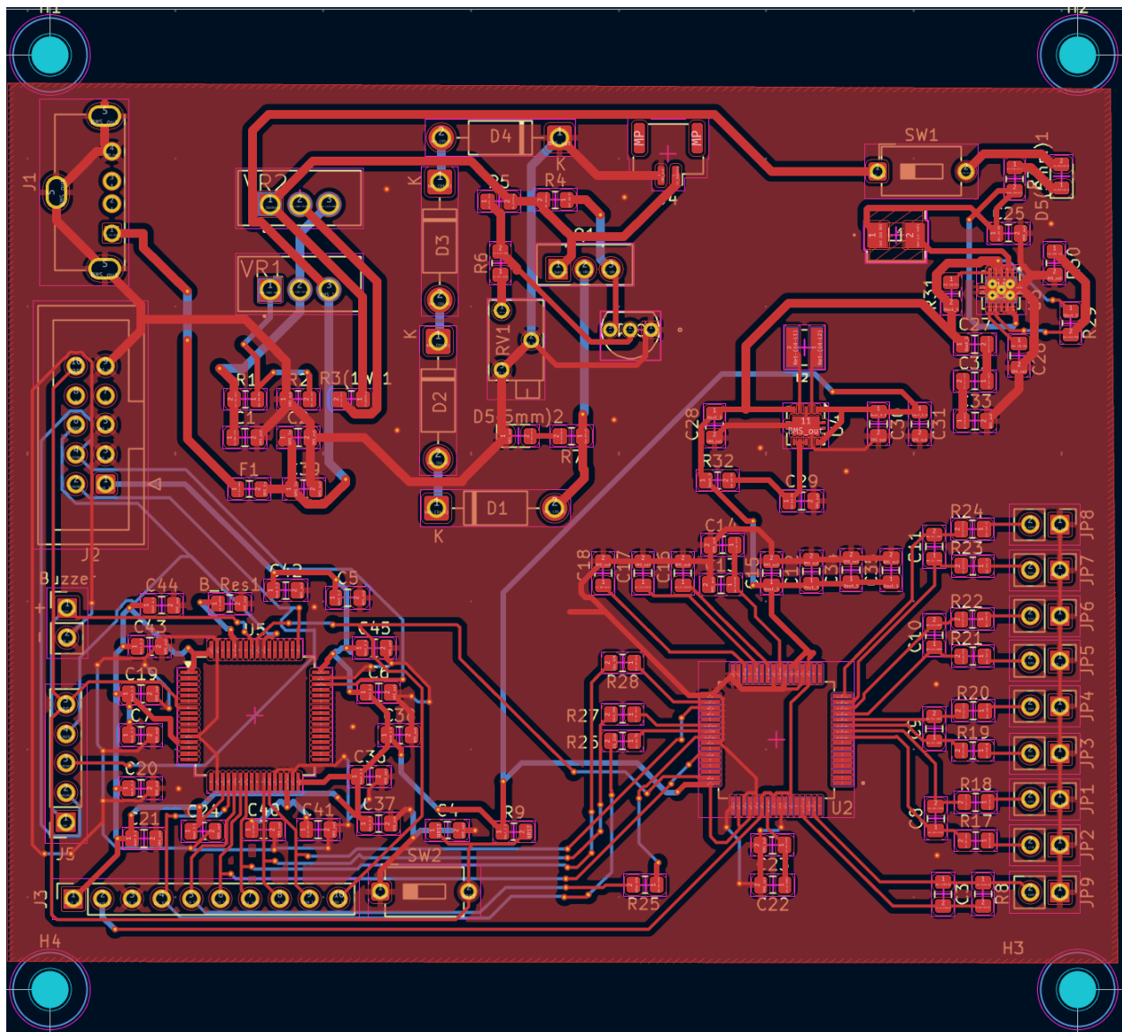
Figure 21: Final PCB design
