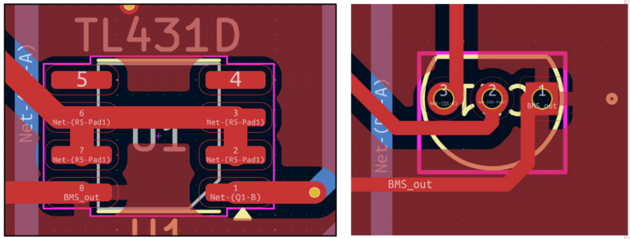
Figure 18: PCB design change for TL431D shunt voltage regulator footprint, old(left) to new(right)
