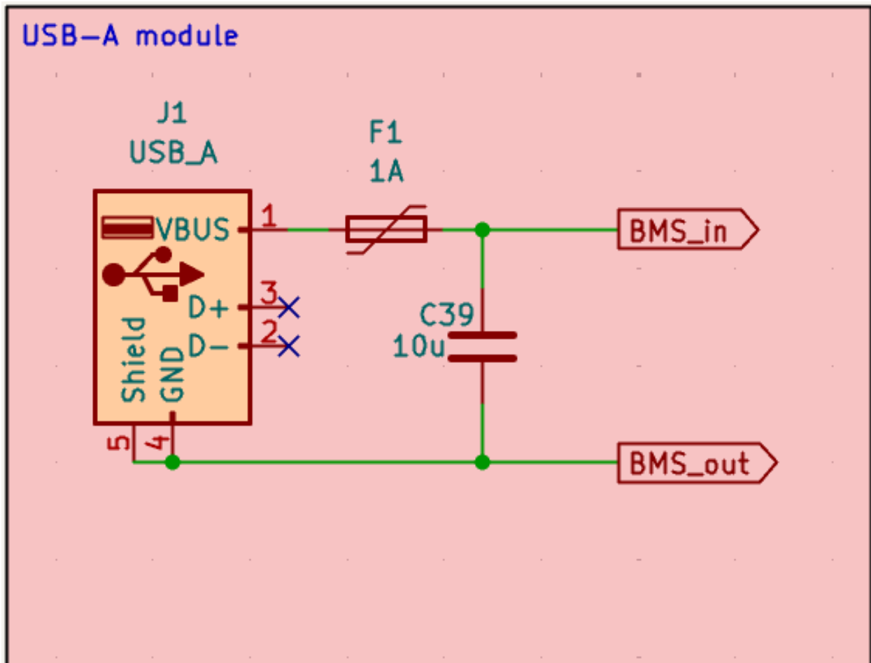
Figure 9: USB-A module schematics
