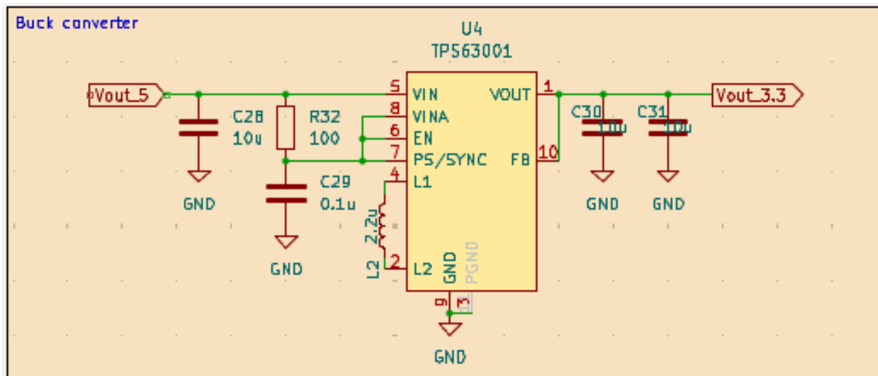
Figure 12: Buck converter schematics
