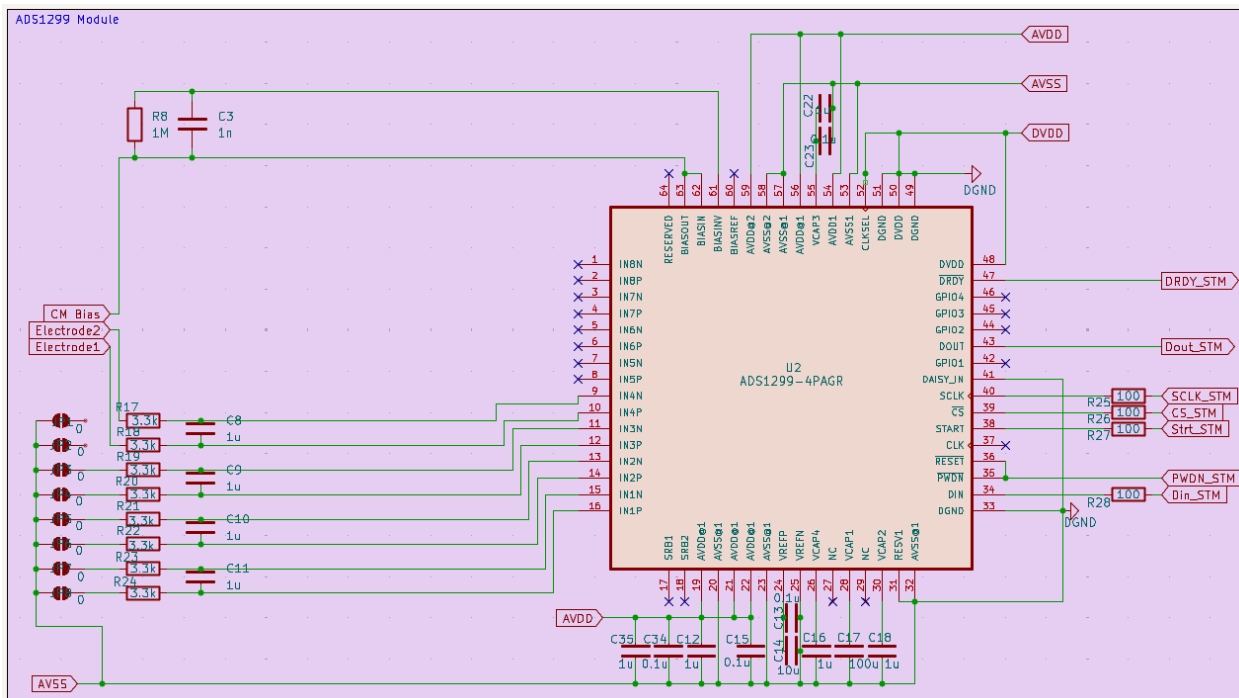
Figure 13: ADS1299 module schematics
