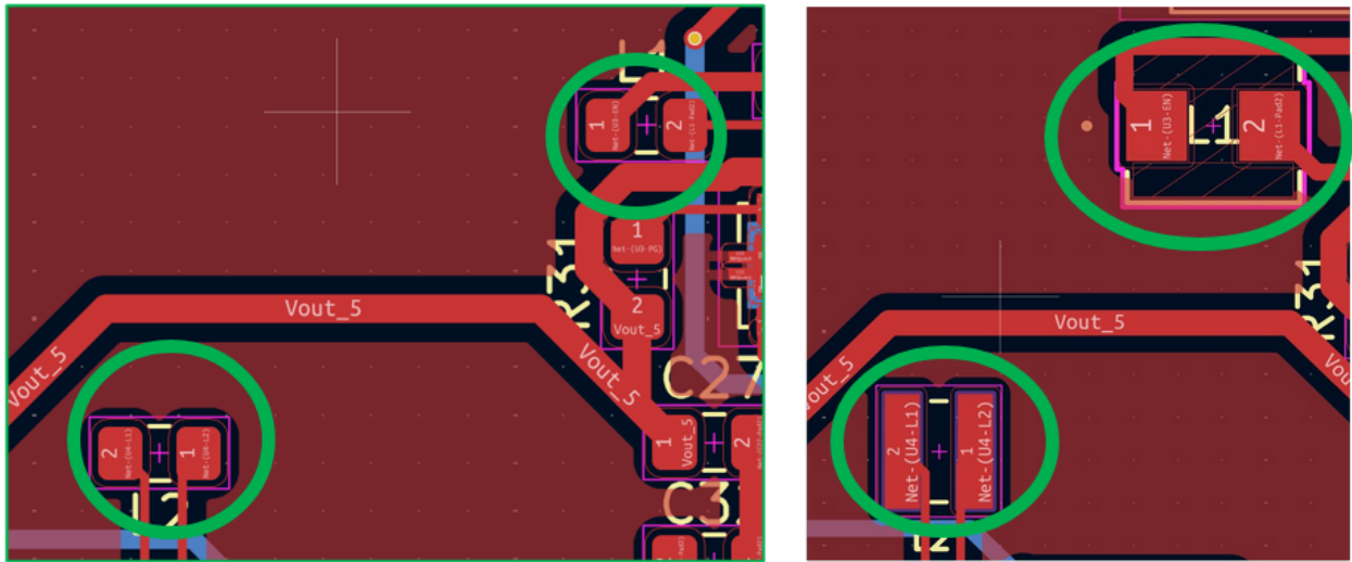
Figure 20: PCB design change to accommodate bigger inductor for power converters, old(left) to new(right)
