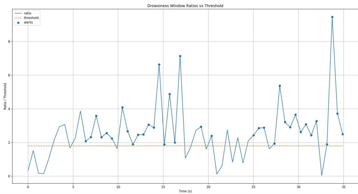
Figure 26: Drowsiness Window VS threshold for Arushi
