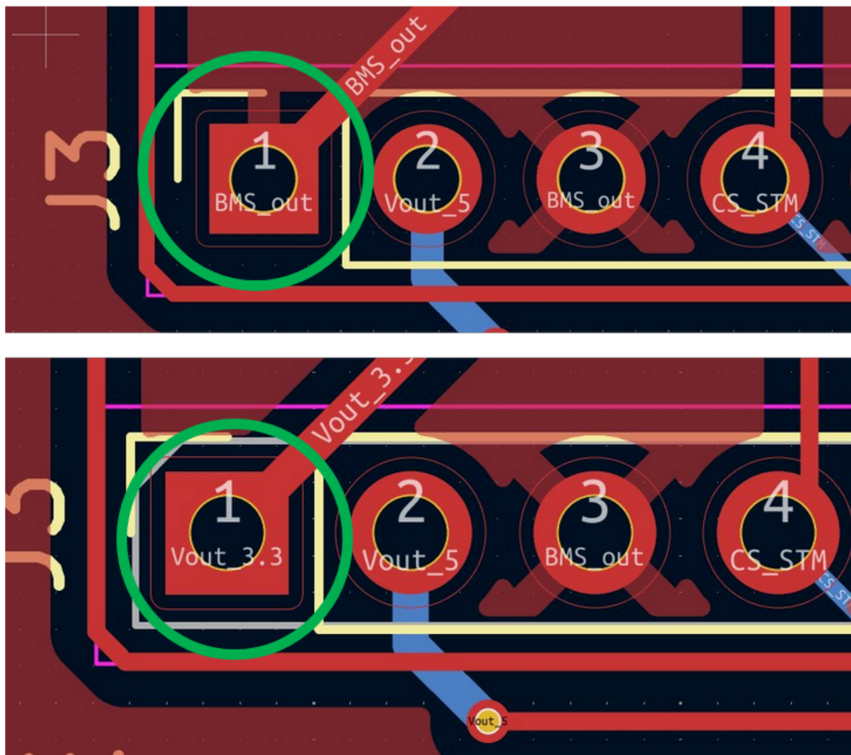
Figure 19: PCB design change to prevent connection mismatch, shorting ground to 3.3V rail, old(above) to new(below)
