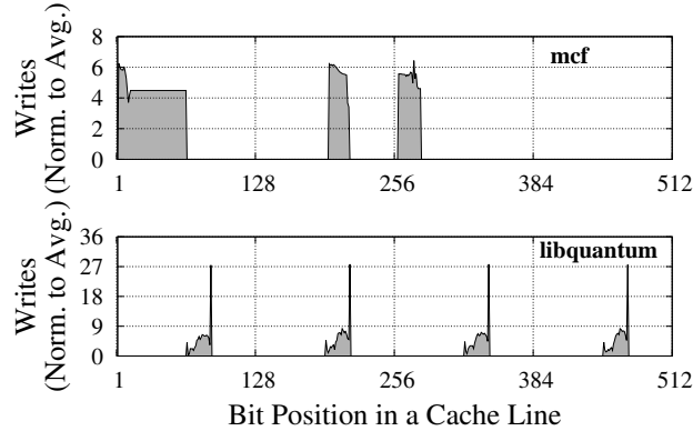
Figure 12. Variation in writes per bit position of a line. The most frequently written bit receives as much as 6x (for mcf ) to 27x (for libquantum ) more writes than average.
