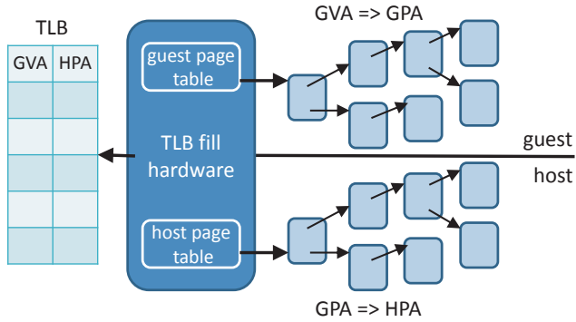
Figure 1. TLB translates guest virtual address (GVA) to host physical address (HPA), disregarding guest physical address (GPA). Upon a miss, the TLB fill hardware finds the missing translation by walking the guest and host page tables to translate GVAs to GPAs and GPAs to HPAs, respectively. The hardware delivers a page fault to the host if it encounters a non-present GPA \Rightarrow HPA, allowing the host to fault-in the missing guest page, on demand. (Reproduced from [16].)
