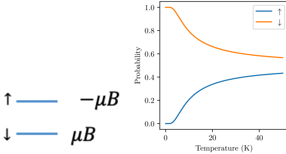
Figure 2: (left) The energy level diagram for a two-state system of an electron in a magnetic field. (right) The probability of each state as a function of temperature.
