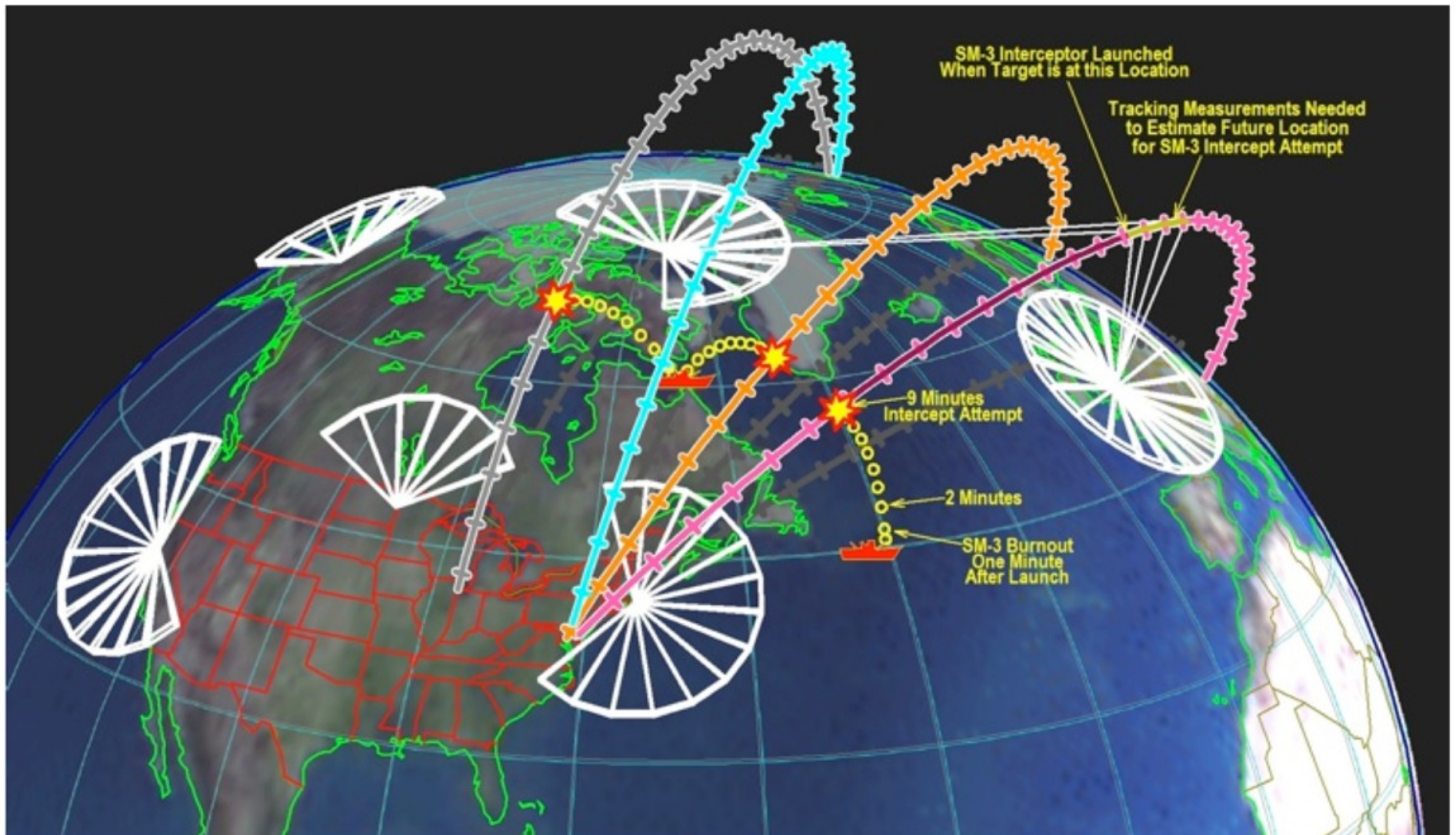
Figure 3: Northwest Atlantic-based SM3 Block II interceptors (with a conservative assumed burnout speed of 4 km/sec) engaging Russian ICBM warheads: each tick on the trajectories marks one minute. ©2018
