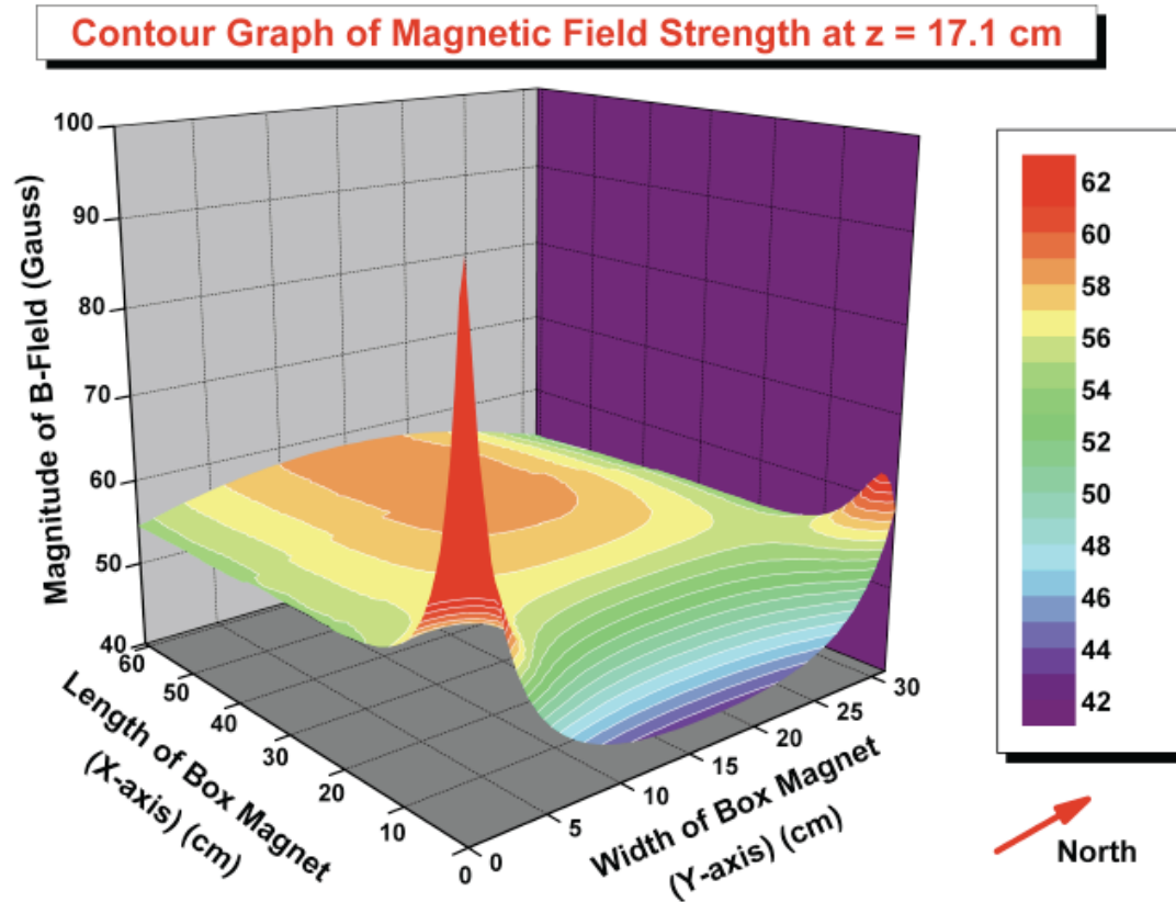
Figure 1.8 Contour graph of magnetic field strength within box magnet. The origin is at the South East corner of the box magnet. Magnitudes above 62 Gauss are colored in red.
