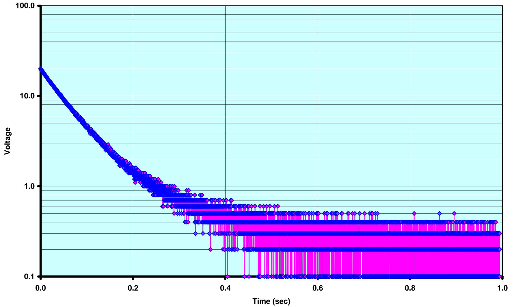
0.05 uF 600V Astron Capacitor Vfg = 10V, f = 50 mHz Square Wave, R_load = 1 Megohm
