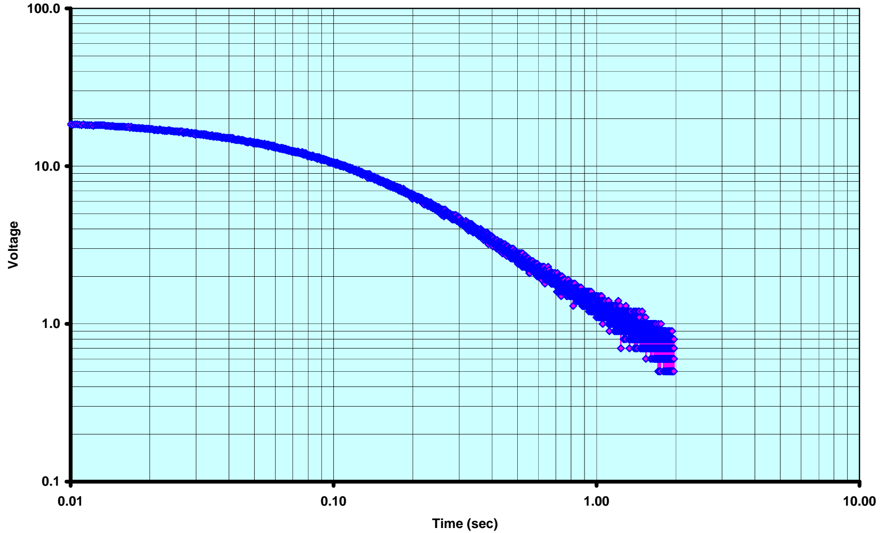
0.1uF 600V Bumblebee Capacitor Vfg = 10V, f = 50 mHz Square Wave, R_load = 1 Megohm
