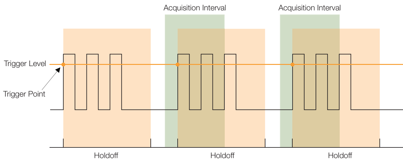
Figure 36. Trigger holdoff.
