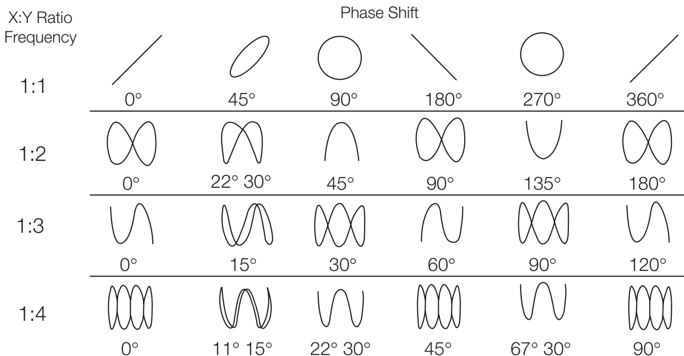
Figure 70. Lissajous patterns.
