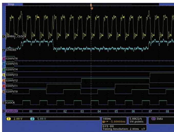
Figure 17. The MSO provides 16 integrated digital channels, enabling the ability to view and analyze time-correlated analog and digital signals.
