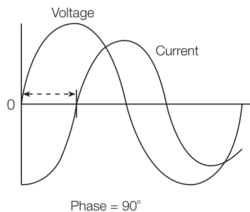
Figure 10. Phase shift.
