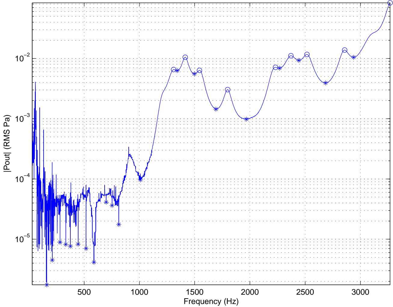
|Pout| Resonance Maxima & Minima
