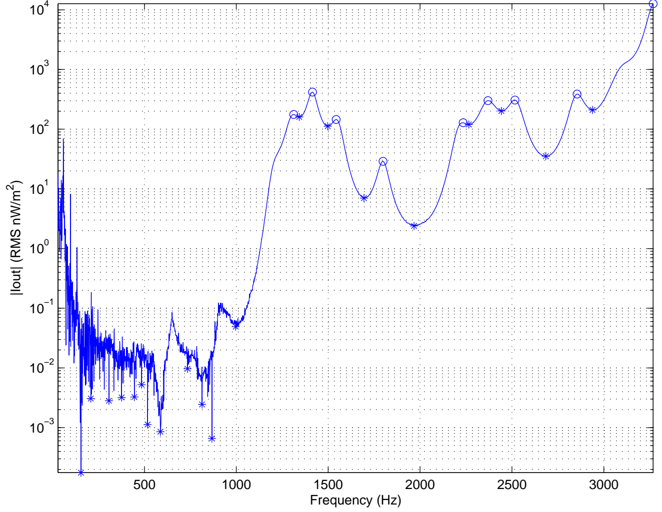
|Iout| Resonance Maxima & Minima
