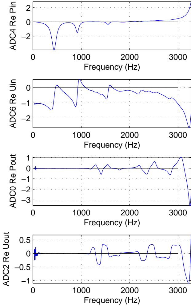
Raw ADC Data (RMS Volts)
