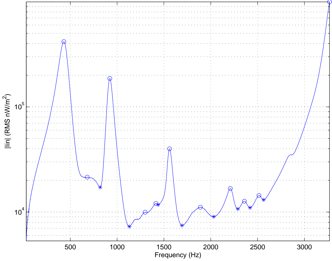
|lin| Resonance Maxima & Minima
