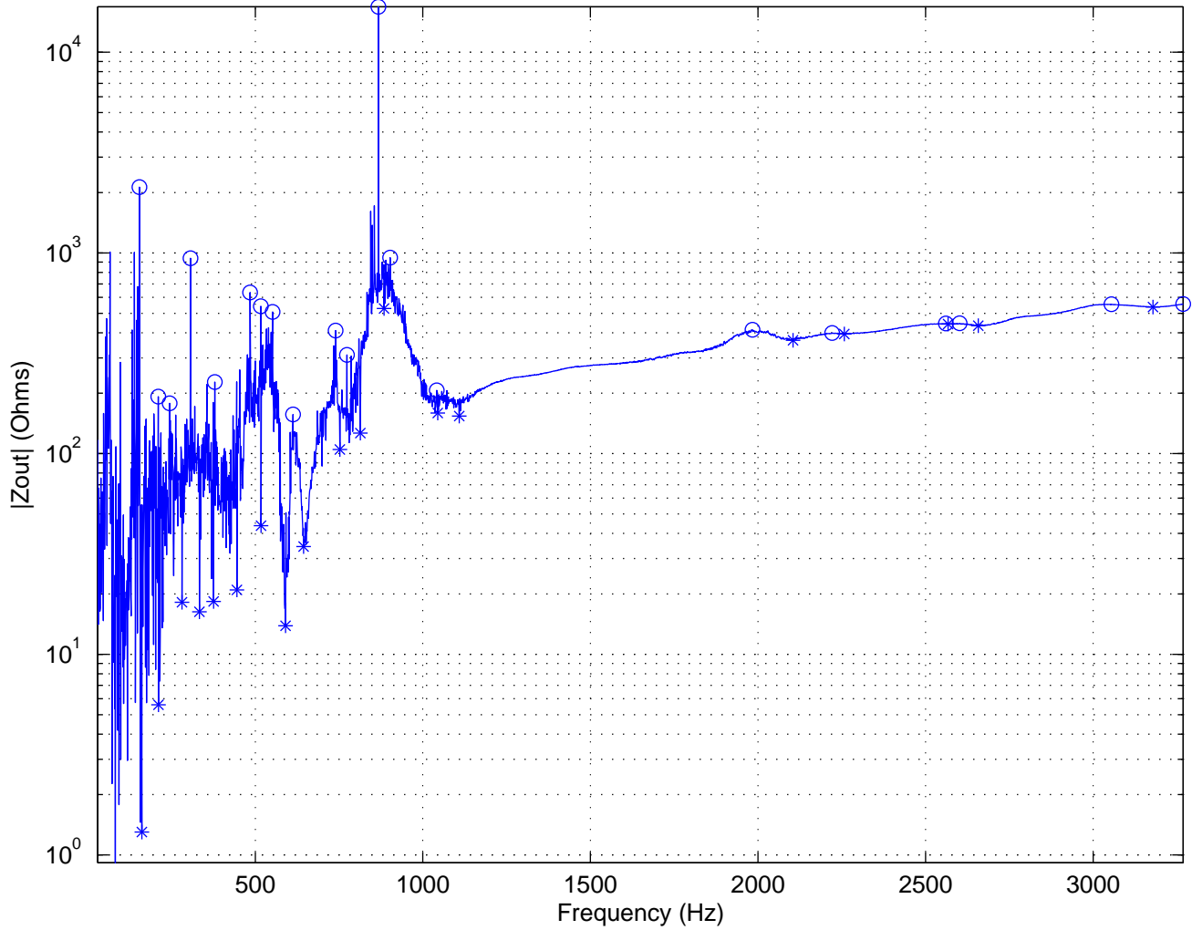
|Zout| Resonance Maxima & Minima
