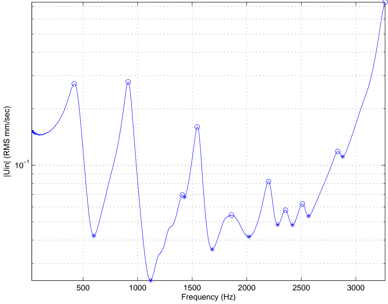
|U in | Resonance Maxima & Minima
