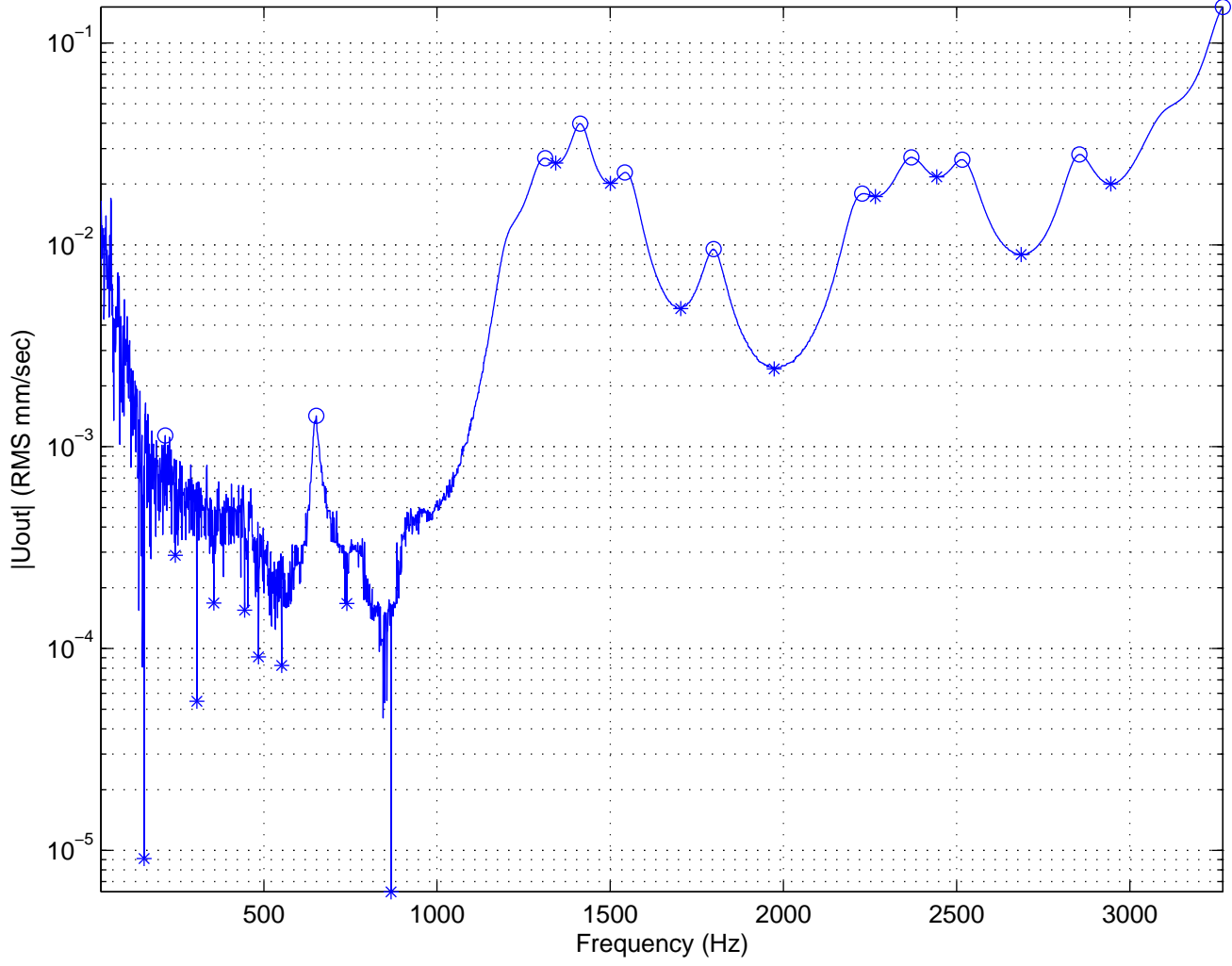
|Uout| Resonance Maxima & Minima
