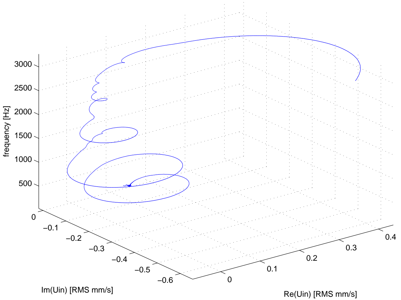
Uin in the Complex Plane
