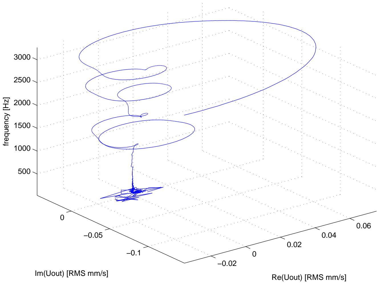
Uout in the Complex Plane
