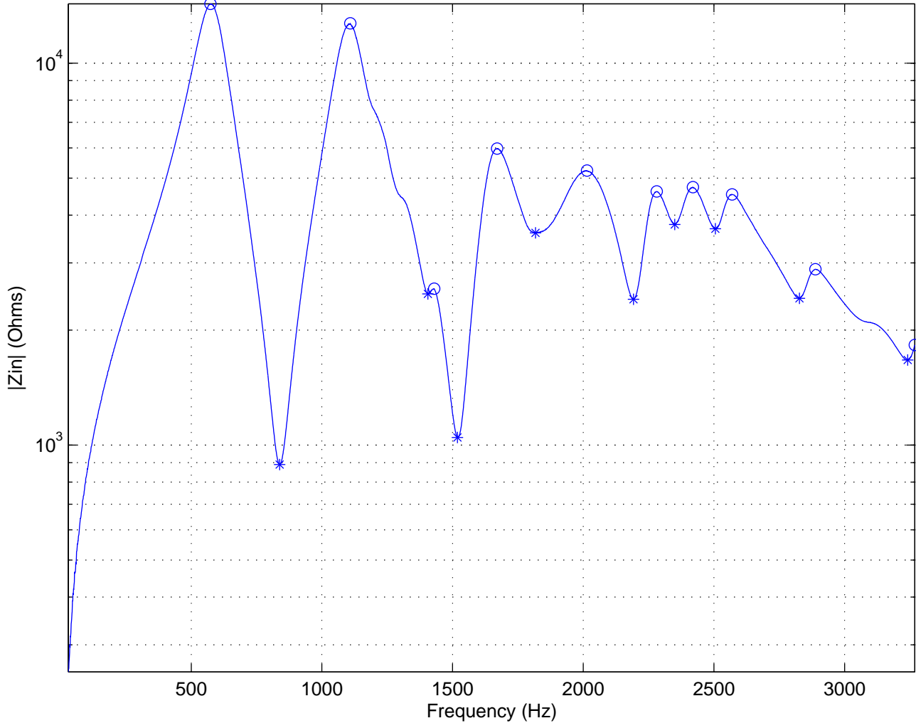
|Zin| Resonance Maxima & Minima
