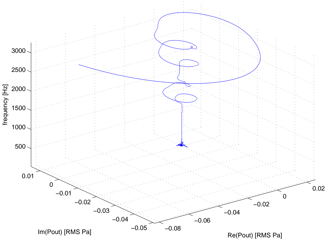
Pout in the Complex Plane
