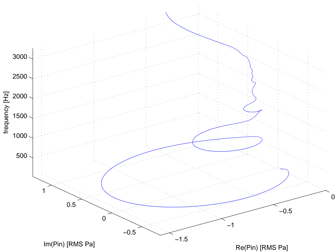
Pin in the Complex Plane
