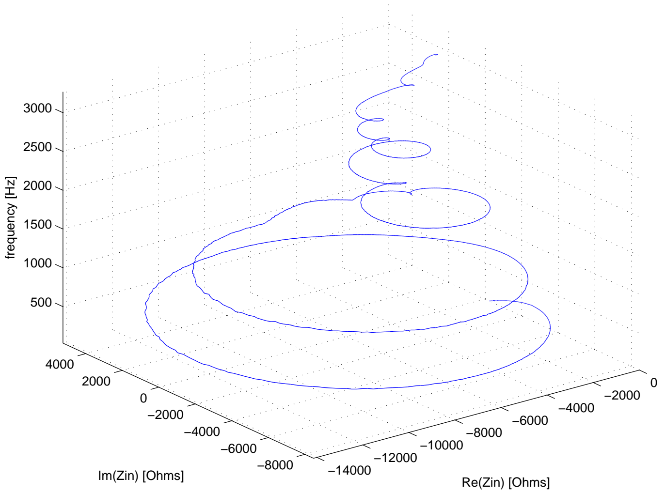
Zin in the Complex Plane
