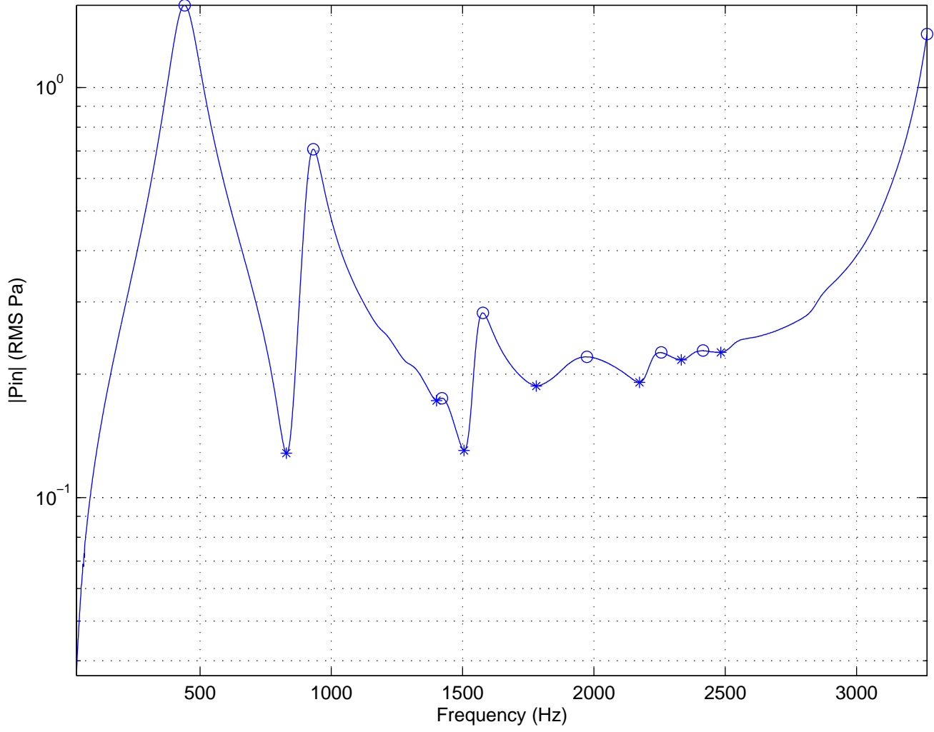
|Pin| Resonance Maxima & Minima
