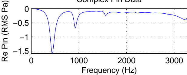
Complex Pin Data
