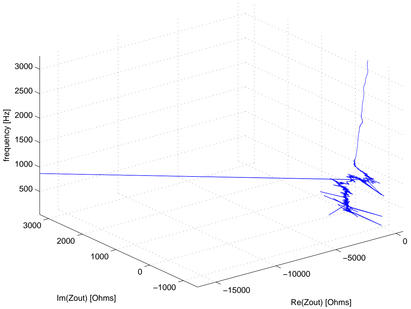
Zout in the Complex Plane
