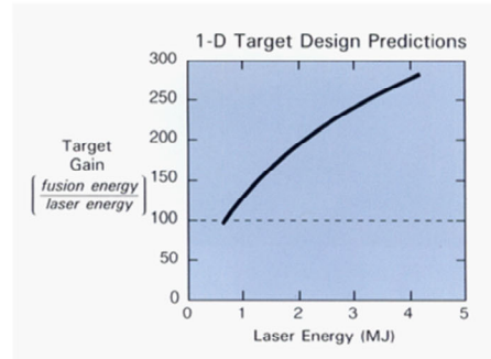
Figure 3. Plot of target gain as a function of input laser energy; the dotted line indicates the minimum gain required for fusion reactor applications.
